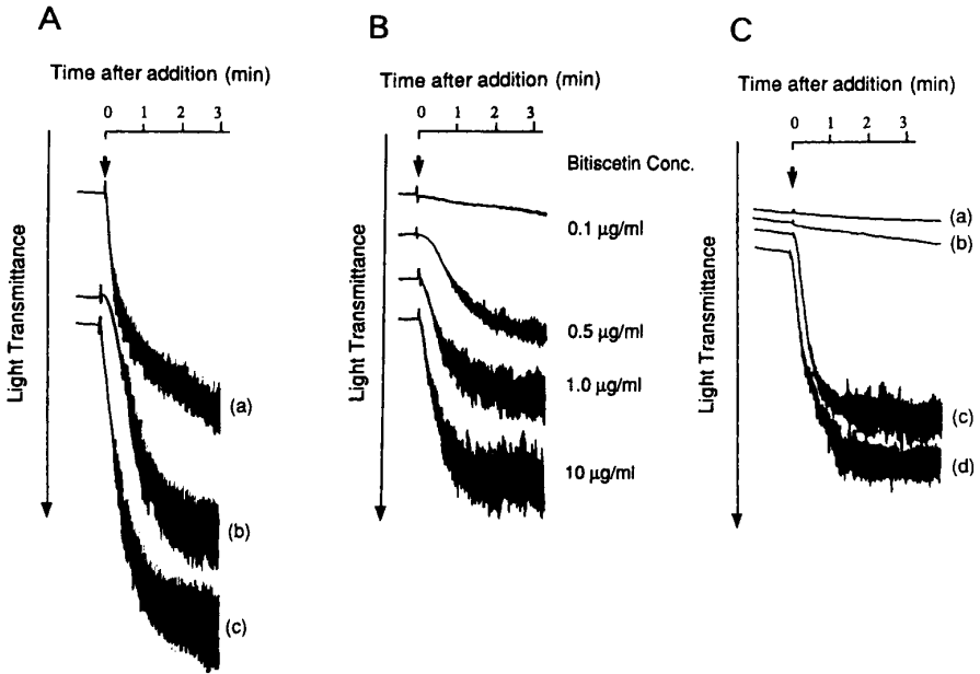
FIG. 3. Platelet agglutination induced by bitiscetin and vWF. (A) PRP ( 3 \times 10^8 platelets/ml) was incubated with 9.2 \mu\text{g/ml} of botrocetin (a), 1 mg/ml of ristocetin (b) and 4.5 \mu\text{g/ml} of bitiscetin at time 0 (arrow). (B) Bitiscetin at various concentrations was added to formalin-fixed platelets ( 3 \times 10^8 /ml in TBS) in the presence of vWF (5 \mu\text{g/ml} ) at time 0 (arrow). (C) Bitiscetin (5 \mu\text{g/ml} ) was added to washed normal platelets ( 3 \times 10^8 /ml) containing vWF (10 \mu\text{g/ml} ) in the presence of 10 \mu\text{g/ml} of B. jararaca GPIIb-BP (a), anti-vWF mAb (NMC-4) (b), anti-GPIIb/IIIa mAb (LJ-CP8) (c) or none (control) (d) at time 0 (arrow).
